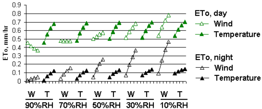
Figure 11. Effect of low (inadequate) airflow rate on evapotranspiration (ET o ). Wind speeds are 1, 3, 5, 7 and 9 m/s (2.2 to 20.1 miles/hr) with constant 30C (86F). Air temperatures are 30, 40, 50, and 60C (86 to 140F) with constant 1 m/s (2.2 miles/hr). There are five sets of wind and temperature data, corresponding to five vapor pressures equivalent to 90%, 70% 50%, 30% and 10%RH at 30C.
